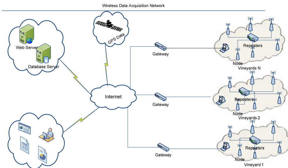
Fig 1: A schematic diagram of WSN layout for modeling the influence of climate change in weather, atmospheric and environmental conditions and on grapevine varieties as well as wine quality in different styles. The WSN transmits real time data collected through remote, wireless telemetry devices via repeaters, gateways and the Internet to a central sever for display and comparative analysis on the variability in climate change across the world's major wine regions and grapevine varieties.
