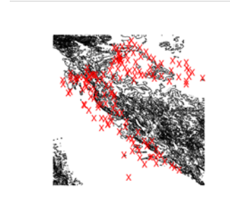
Figure 2. A digital elevation model for Croatia with superimposed weather station locations
