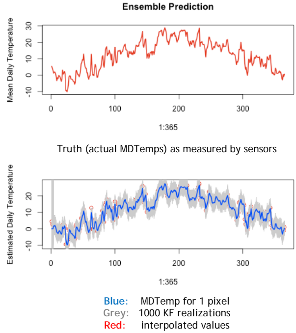
Figure 2. EnKF model compared with truth
